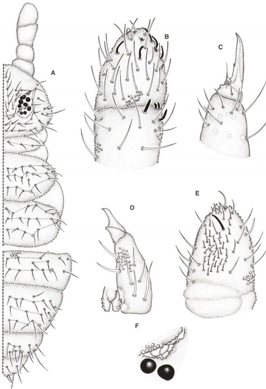
Fig.54 : Superodontella lamellifera Axelson, 1903.
