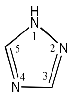
1, 2,4-triazole
