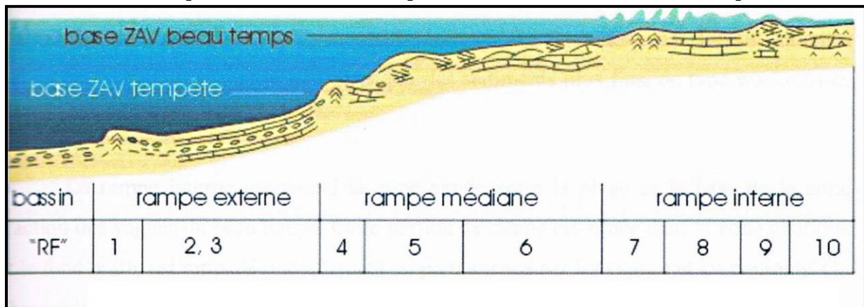
Fig.63: Microfaciès standards de rampe, Boulvain, 2008.
